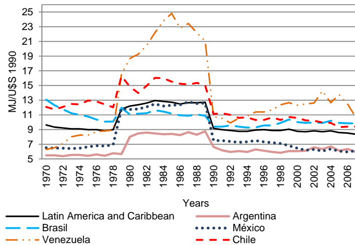
Figure 1: Energy intensity of final energy consumption of Latin America and Caribbean region and countries. 1970-2007
