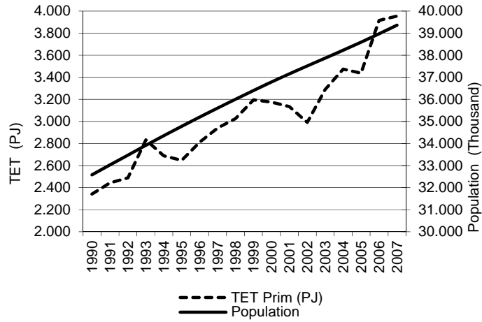
Figure 6: Population and TET evolution. 1990-2007
