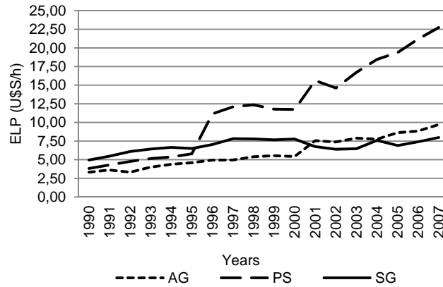
Figure 9. ELP AG , ELP PS , and ELP SG evolution. 1990-2007
