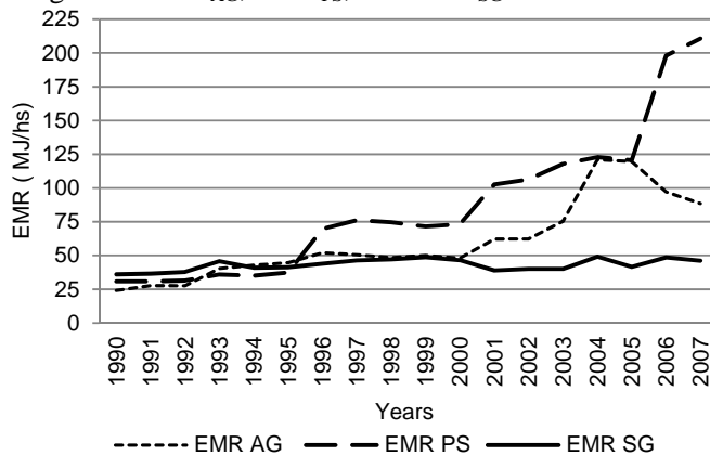
Figure 8. EMR_{AG} , EMR_{PS} , and EMR_{SG} evolution. 1990-2007
